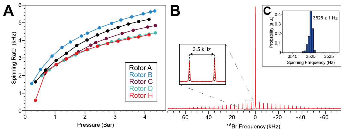
Figure 3. Spin test data. A.) Spinning rate as a function of applied air pressure for rotors A, B, C, D, and H. B.) ^{79}\text{Br} spectrum of KBr packed into rotor H and spinning at 3.5 kHz at the magic angle; 512 scans. C.) Histogram of spinning frequencies without spinning regulation over the 10 minute KBr data acquisition period.
