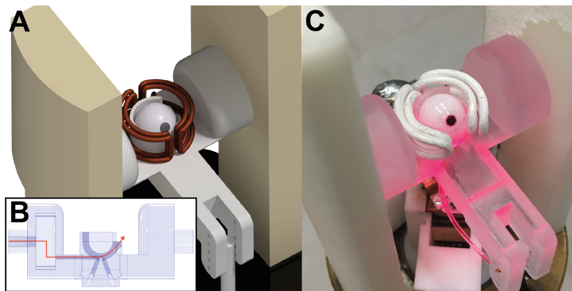
Figure 1. Experimental apparatus. A.) Probehead design schematic depicting the stator with a double saddle coil, spherical rotor, and angle adjust arm. B.) Cross-section view of the stator showing the drive gas inlet and angled through holes for the fiber optic tachometer. Drive gas is fed from the left side into the stator cup (red arrow). C.) Fully assembled probehead.
